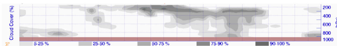
Figure 4. Cloud chart with 6 day forecast. Cloud cover in 5 classes (as % of total sky cover). Ground level as average of surrounding area.
